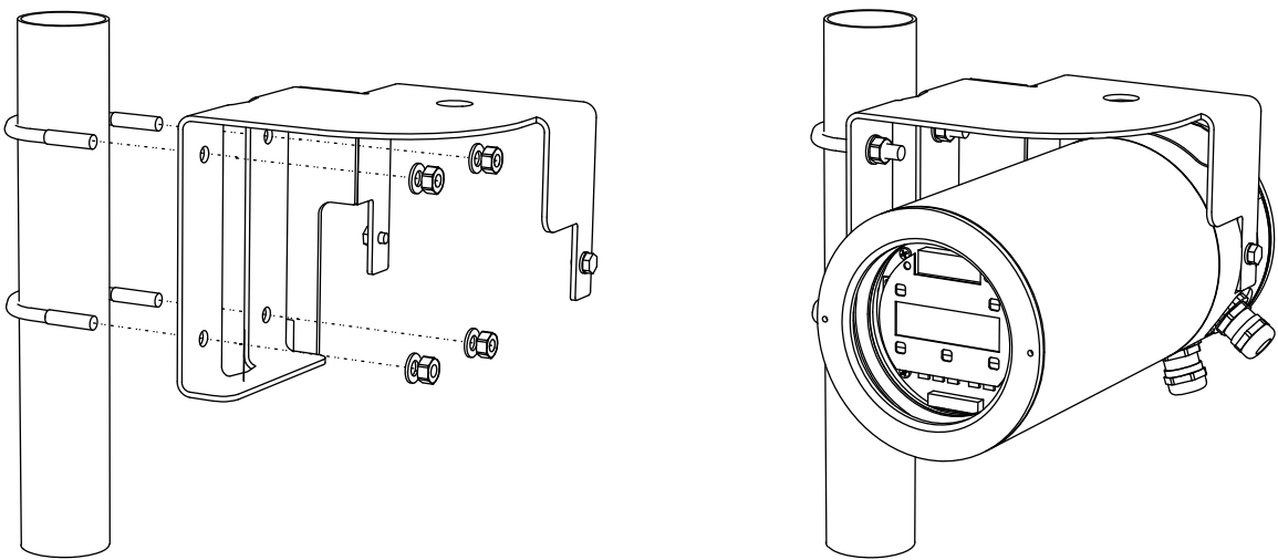
FLUXUS ADM 8127
